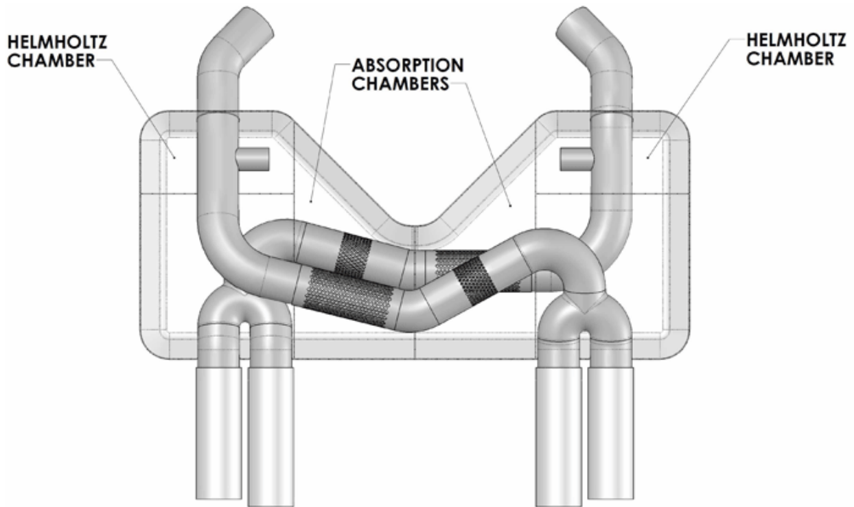
E90/E92 M3 STOCK REAR MUFFLER
