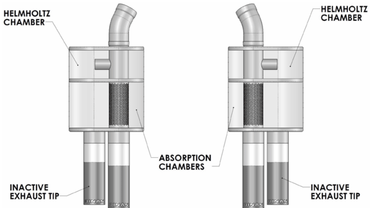
E90/E92 M3 DINAN MUFFLERS
