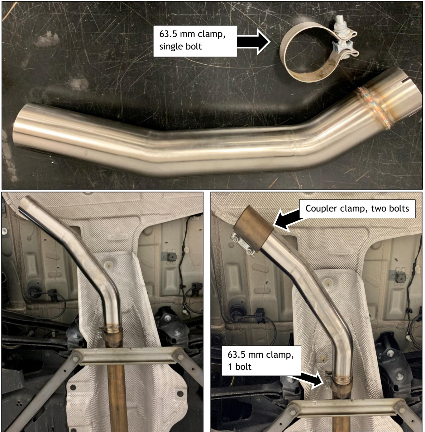
Figure 7: Assembly: Inlet Tube Installation
